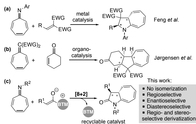
Scheme 1. Enantioselective versions of [8+2] cycloaddition.
