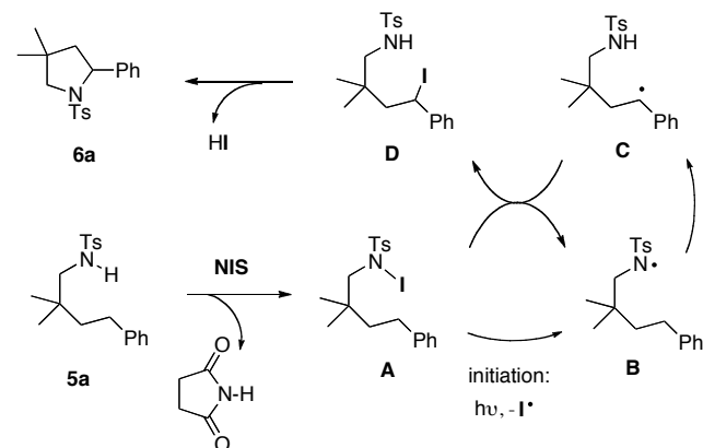
Figure 1. Mechanistic scenario for NIS-promoted Hofmann-Löffler reaction.
