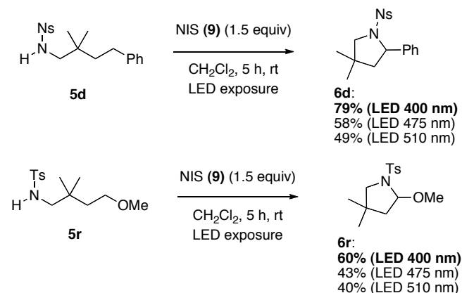
Scheme 3. LED-initiated Hofmann-Löffler reaction.
