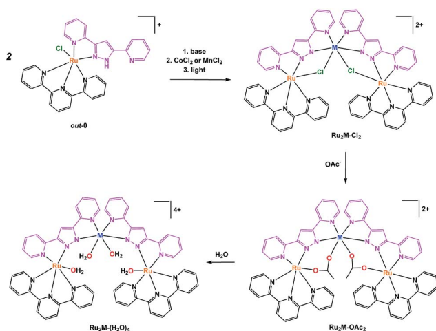
Scheme 1 Synthetic strategy followed for the preparation of trinnuclear complexes and their labelling.
