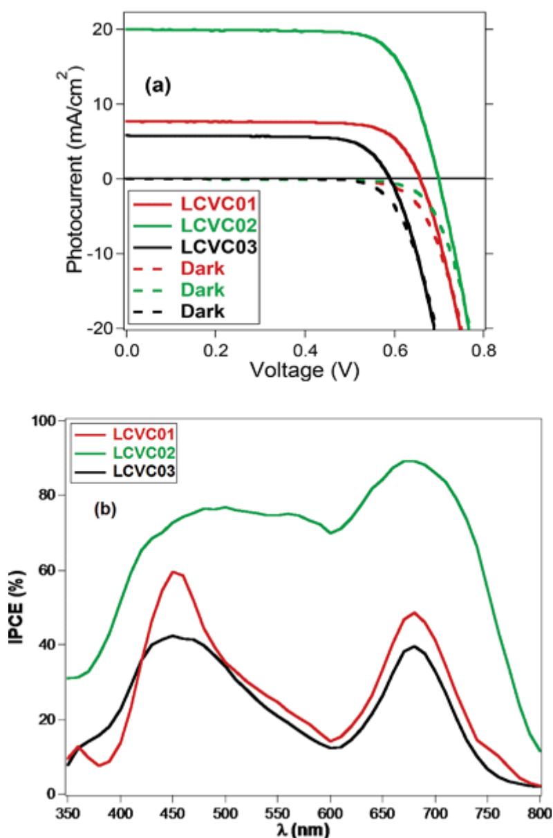
Fig. 5 (a) I - V curves for LCVC01 , LCVC02 and LCVC03 ; and (b) IPCE spectra of LCVC01 , LCVC02 and LCVC03 . DSSC devices recorded under AM 1.5G radiation. The dashed lines correspond to the I / V dark curves.
