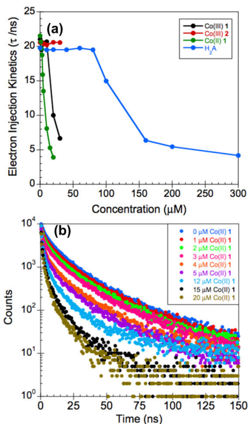
Figure 3. (a) Electron transfer lifetime as function of the cobalt complex and H 2 A concentration. The electron transfer lifetime was calculated following a reported methodology. 27 (b) Time resolved photoluminescence of colloidal CdTe QDs upon addition of increasing amounts of Co(II)-1. The samples were excited at \lambda_{\text{ex}} = 405 nm and monitored at \lambda_{\text{em}} = 600 nm. [CdTe QDs] = 2 \mu\text{M} . 28
