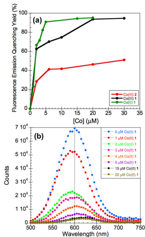
Figure 2. (a) Quenching emission yield as function of complex concentration. (b) Steady state photoluminescence of colloidal CdTe QDs upon addition of increasing amounts of Co(II)-1. The samples were excited at \lambda_{ex} = 405 nm. [CdTe QDs] = 2 \mu\text{M} . 28
