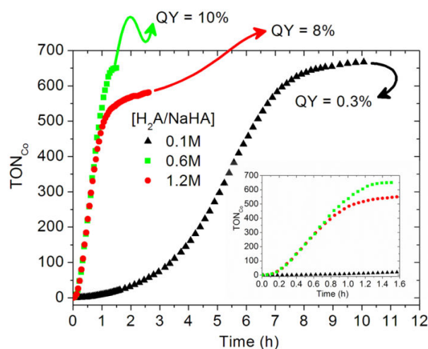
Figure 5. Photocatalytic hydrogen production experiments were performed using an aqueous mixture of [\text{CdTe QDs}] = 5.9 \times 10^{-5} M, [\text{Co(III)-1}] = 7.5 \times 10^{-5} M and [\text{H}_2\text{A}/\text{NaHA}] = 0.1 M ( \blacktriangle ), 0.6 M ( \blacksquare ) or 1.2 M ( \bullet ), pH = 4.1, volume = 1.5 mL, under 1 sun irradiation ( \lambda > 400\text{nm} ). Inset: Expanded graph (0-1.6h). Turnover Number ( \text{TON}_{\text{Co}} ) = mol \text{H}_2 /mol cobalt, average of two different replicates (within 5-10 % error, see also Figure S9). Values of quantum yield (QY) for each experiment are given at maximum conversion time and were calculated as \text{QY} = [2 \times (\text{molecules of H}_2)] / [\text{photons absorbed} \times \Delta t \times \text{Area}] , see also Figure S10.
