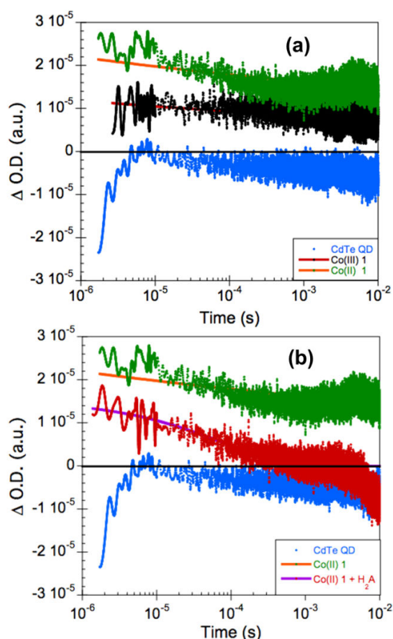
Figure 4. Transient absorption decays of colloidal CdTe QDs (a) upon addition of 30 \mu\text{M} of Co(III)-1 or Co(II)-1. (b) upon addition of 30 \mu\text{M} of Co(II)-1 and 250 \mu\text{M} of \text{H}_2\text{A} . The samples were excited at \lambda_{\text{ex}}=430 nm and the decays were monitored at \lambda_{\text{probe}}=675 nm. [\text{CdTe QDs}] = 2 \mu\text{M} . 28 The orange, red and purple lines in the plots indicate the experimental points' trend that was obtained by fitting the data to the power law function indicated in equation (1).
