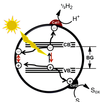
Figure 1. Schematic representation of photo-driven hydrogen generation at a semiconductor. Black Arrows: Light excitation, charge migration (electrons = \ominus , holes = \oplus ) and catalytic reactions. Red Arrows: photoluminescence and charge recombination. CB = Conduction Band, VB = Valence Band, BG = Band-Gap. S/Sox = substrate/oxidized substrate. Cat1 = catalyst for water reduction. Cat2 = catalyst for substrate oxidation.
