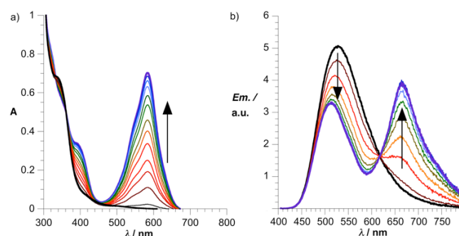
Figure 3. UV-vis absorption (a) and emission (b) spectral changes of K Sn [BSPR] in acetonitrile solution (4.10 -5 M, T = -30°C) during photoirradiation (335 nm). Black curves correspond to the spectra of K Sn [BSPR] before irradiation; purple curves correspond to the spectra of the sample in the photolysis steady-state.
