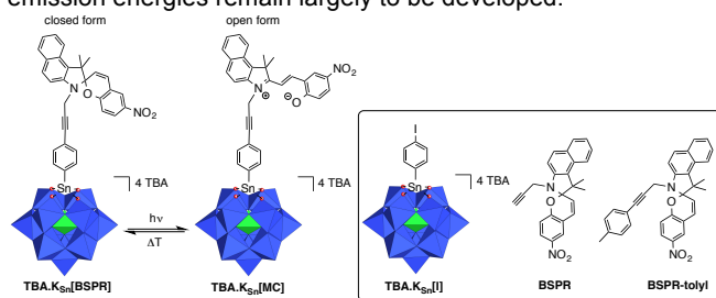
Figure 1. Photoisomerization process occurring in the organo-tin POM hybrid K_{Sn}[BSPR] . Framed: Molecular representation of the reference compounds K_{Sn}[I] , BSPR and BSPR-tolyl described in this study
