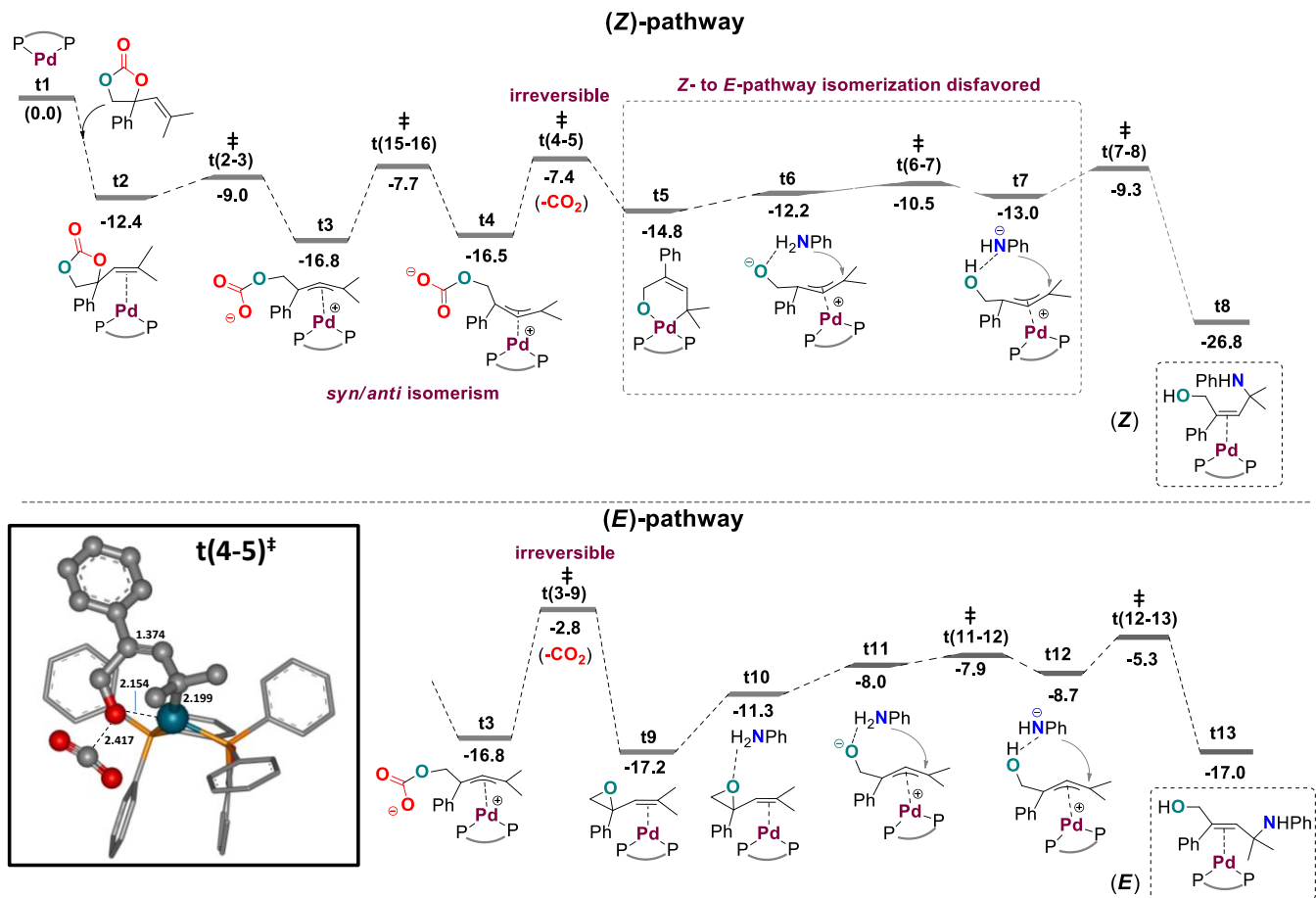
Figure 8. Computed free energy profile (in kcal/mol) for the synthesis of allylic amine product 40 reported in Figure 4. The structure of the transition state leading to t5 (i.e., t(4-5) ‡ ) is shown in the inset with selected calculated bond lengths.
