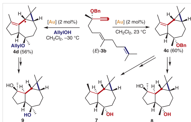
Scheme 4 Gold(I)-catalyzed total synthesis of aromadendranes. [\text{Au}] = [(\text{JohnPhos})\text{Au}(\text{MeCN})]\text{SbF}_6 .
