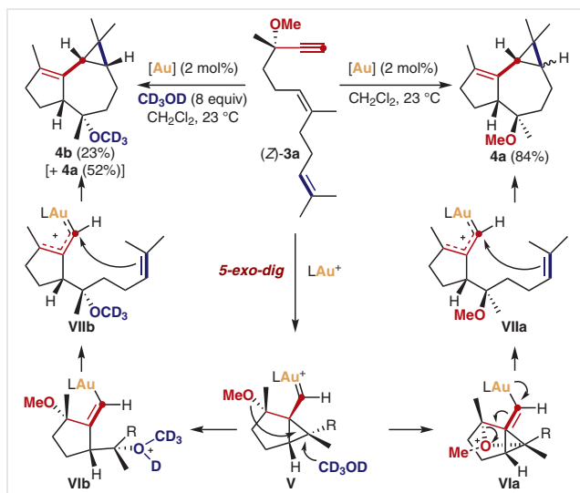
Scheme 2 Gold(I)-catalyzed tandem cyclization/1,5-OR migration/intramolecular cyclopropanation of dienes. [\text{Au}] = [(\text{JohnPhos})\text{Au}(\text{MeCN})]\text{SbF}_6 .
