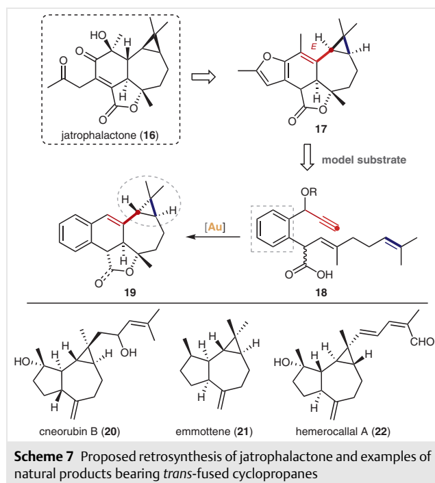
Scheme 5 Intramolecular gold(I)-catalyzed [2+2+2] alkyne/alkene/carbonyl cycloaddition of oxo-1,6-enynes. [Au] = AuCl.
