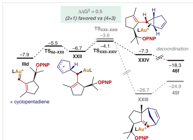
Scheme 20 DFT calculations for the intermolecular trapping of IIIc with cyclopentadiene. L = JohnPhos; PNP = p -nitrophenyl.
