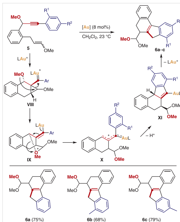
Scheme 3 A 1,6-shift of the MeO group in the cyclization of 1,7-enynes catalyzed by gold(I). [\text{Au}] = [(\text{JohnPhos})\text{Au}(\text{MeCN})]\text{SbF}_6 .
