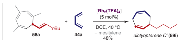
Scheme 29 Total synthesis of dictyoptereene C' by (4+3) cycloaddition
