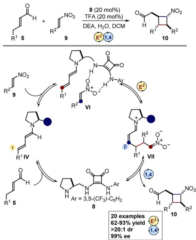
Scheme 3. E^2 -1,4 cascade reaction: use of a two-carbon electrophile 9 to access cyclobutanes 10 by means of a vinyllogous formal [2 + 2] reaction. E^2 : dienamine; 1,4: iminium ion; the blue circle represents the chiral scaffold of catalyst 8 . DEA: diethylamine; TFA: trifluoroacetic acid.
