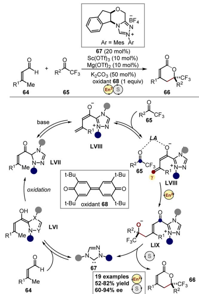
Scheme 20. The first reported use of NHC catalysis to develop a vinyllogous cascade; En^2/S cyclization pathway. En^2 : vinyllogous enolate; S: spontaneous cyclization. The blue and grey circles represent the chiral scaffolds of the NHC catalyst 67 . The reactive carbon atoms are highlighted in different colors, depending on their inherent reactivity: magenta stands for a nucleophilic position, and blue for an electrophilic center.
