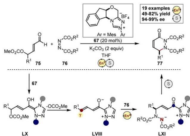
Scheme 23. NHC-mediated \text{En}^2 -S cascade sequence; \text{En}^2 : vinylogous enolate; S: spontaneous cyclization. Formation of the vinylogous enolate achieved via Strategy 3 in Figure 10.
