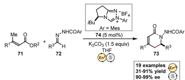
Scheme 22. NHC-mediated En^2 -S cascade sequence; En^2 : vinyllogous enolate; S: spontaneous cyclization. Formation of the vinyllogous enolate achieved via Strategy 2 in Figure 10.
