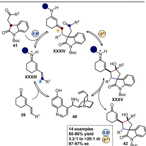
Scheme 13. The first report of a 1,6-E 2 cascade sequence; 1,6: vinylogous iminium ion; E 2 : dienamine. The blue circle represents the chiral scaffold of the cinchona-based primary amine catalyst. The reactive carbon atoms are highlighted in different colors, depending on their inherent reactivity: magenta stands for a nucleophilic position, and blue for an electrophilic center.
