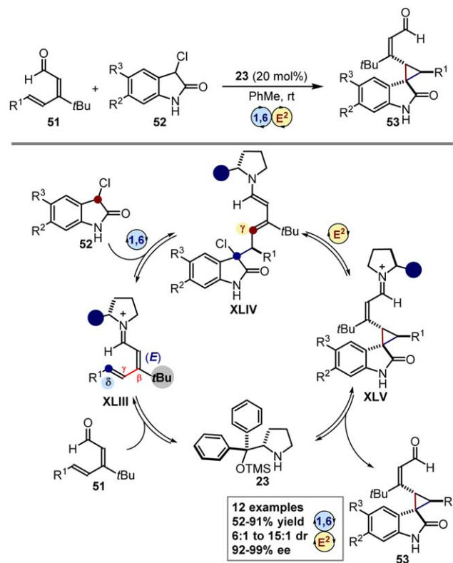
Scheme 16. Synthesis of cyclopropane spiro-oxindoles 53 by means of a 1,6-E 2 cascade reaction with linear dienals; 1,6: vinyllogous iminium ion; E 2 : dienamine. The blue circle represents the chiral scaffold of the aminocatalyst 23 . The grey circle in XLIII highlights the importance of the tert -butyl moiety as a steering group.
