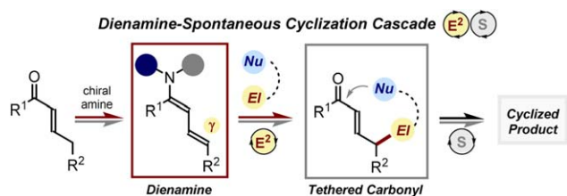
Fig. 5. Dienamine ( E^2 )/spontaneous (S) non-catalyzed cyclization cascade pathway; the blue and grey circles represent the chiral scaffolds of the aminocatalyst.
