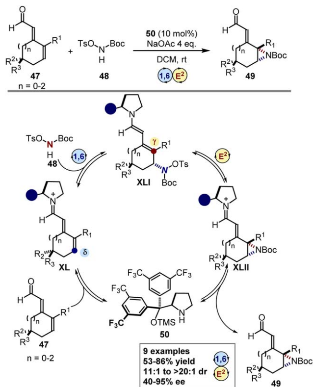
Scheme 15. Remote aziridination of cyclic enals by means of a 1,6-E 2 cascade reaction; 1,6: vinyllogous iminium ion; E 2 : dienamine. The blue circle represents the chiral scaffold of the aminocatalyst 50 . The reactive carbon atoms are highlighted in different colors, depending on their inherent reactivity: magenta stands for a nucleophilic position, and blue for an electrophilic center.
