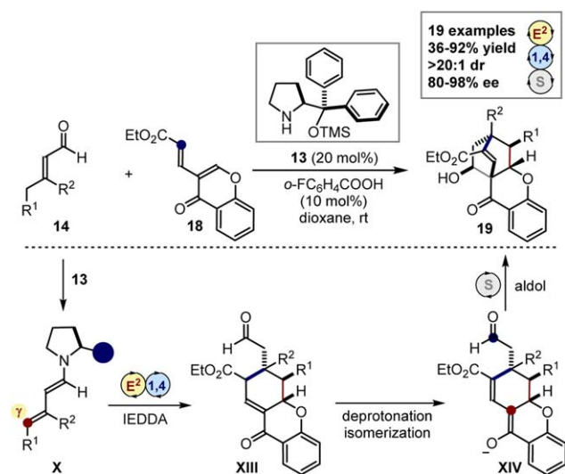
Scheme 6. Dienamine-spontaneous cyclization ( E^2 -S) cascade sequence for the construction of tetracyclic products. The non-catalyzed step is an intramolecular aldol reaction; E^2 : dienamine; 1,4: iminium ion; S: spontaneous step. The reactive carbon atoms are highlighted in different colors, depending on their inherent reactivity: magenta stands for a nucleophilic position, and blue for an electrophilic center.
