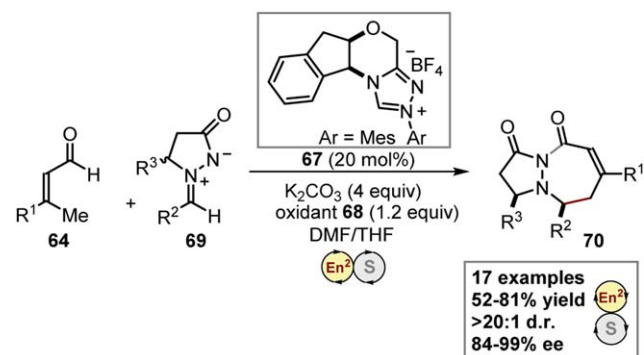
Scheme 21. The formation of the formal [4 + 3] product 70 through a En^2 -S cascade sequence; En^2/S cyclization pathway; En^2 : vinyllogous enolate; S: spontaneous cyclization.
