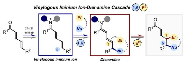
Fig. 8. Vinylogous iminium ion (1,6)/dienamine (E 2 ) cascade pathway; the blue and grey circles represent the chiral scaffolds of the aminocatalyst.
