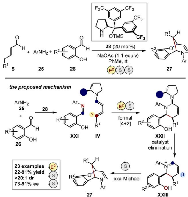
Scheme 9. The formation of structurally complex benzoxazocines 27 through an E^2 -S-S reaction sequence. The non-catalyzed step is an intramolecular oxa -Michael reaction; E^2 : dienamine; S: spontaneous step. The blue circle represents the chiral scaffolds of the aminocatalyst. The reactive carbon atoms are highlighted in different colors, depending on their inherent reactivity: magenta stands for a nucleophilic position, and blue for an electrophilic center.
