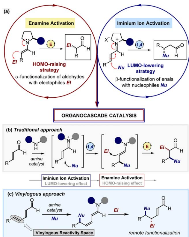
Fig. 1. (a) Combining enamine and iminium ion activations. (b) The established iminium ion-enamine activation strategy for designing organocascade reactions. (c) Transferring the technique into a vinylogous reactivity pattern to forge multiple stereocenters remote from the catalyst's point of action; EI : electrophile, Nu : nucleophile; E : Enamine activation; 1,4: iminium ion-mediated 1,4-addition.
