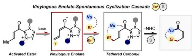
Fig. 11. Vinyllogous enolate ( En^2 )/spontaneous (S) cyclization cascade pathway; the initial organocatalytic event is followed by a spontaneous ipso -cyclization. The blue and grey circles represent the chiral scaffolds of the NHC catalyst.
