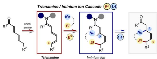
Fig. 6. Trienamine ( E^3 )/iminium ion (1,4) cascade sequence; initial HOMO-raising activation event at the \varepsilon -position, followed by a complementary LUMO-lowering event. The blue and grey circles represent the chiral scaffolds of the aminocatalyst.
