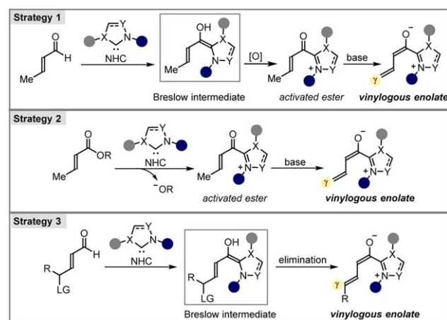
Fig. 10. The different strategies utilized to form vinylogous enolates using NHC catalysis; the blue and grey circles represent the chiral scaffold of the NHC catalyst.
