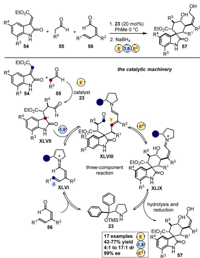
Scheme 17. The vinylogous triple cascade proceeds by way of an enamine (E)/vinylogous iminium ion (1,6)/dienamine activation ( E^2 ) sequence; E: enamine; 1,6: vinylogous iminium ion; E^2 : dienamine. The blue circle represents the chiral scaffold of the aminocatalyst 23 . The reactive carbon atoms are highlighted in different colors, depending on their inherent reactivity: magenta stands for a nucleophilic position, and blue for an electrophilic center.
