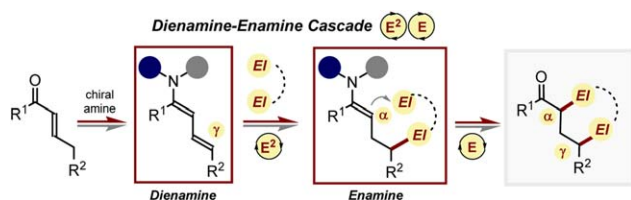
Fig. 4. Dienamine ( E^2 )/enamine (E) cascade sequence; the blue and grey circles represent the chiral scaffolds of the aminocatalyst.
