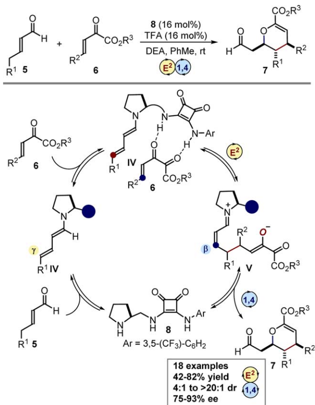
Scheme 2. Synthesis of dihydropyrans 7 through an E 2 -1,4 cascade reaction facilitated by the bifunctional catalyst 8 . E 2 : dienamine; 1,4: iminium ion; the blue circle in IV and V represents the chiral scaffolds of catalyst 8 . The reactive carbon atoms are highlighted in different colors, depending on their inherent reactivity: magenta stands for a nucleophilic position, and blue for an electrophilic center. DEA: diethylamine; TFA: trifluoroacetic acid.
