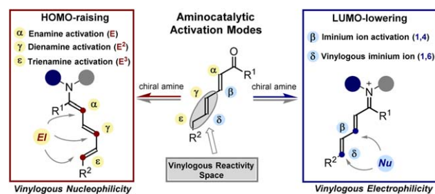
Fig. 2. Established activation modes in aminocatalysis and the possibility of inducing vinylogous nucleophilicity and electrophilicity. The reactive carbon atoms are highlighted in different colors, depending on their inherent reactivity: magenta stands for a nucleophilic position, and blue for an electrophilic center; EI : electrophile; Nu : nucleophile.
