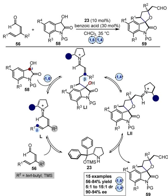
Scheme 18. Synthesis of tetrahydrofuranyl spirooxindoles 59 by means of a 1,6-1,4 cascade reaction with linear dienals; 1,6: vinylogous iminium ion; 1,4: iminium ion. The blue circle represents the chiral scaffold of the aminocatalyst 23 . The grey circle in L highlights the importance of the bulky R^2 substituent as a conformational anchor; TMS: trimethylsilyl; PG: protecting group. The reactive carbon atoms are highlighted in different colors, depending on their inherent reactivity: magenta stands for a nucleophilic position, and blue for an electrophilic center.
