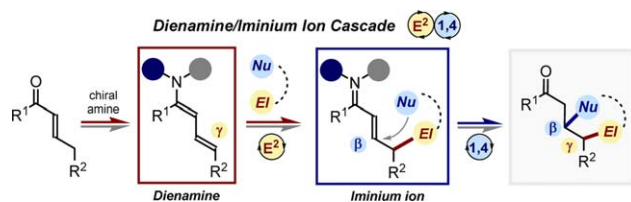
Fig. 3. Dienamine ( E^2 )/iminium ion (1,4) cascade sequence; the blue and grey circles represent the chiral scaffolds of the aminocatalyst.
