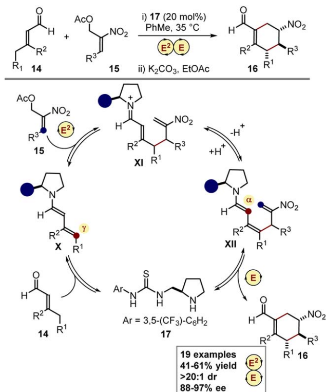
Scheme 5. Functionalization of the \alpha - and \gamma -position of enals 14 through a dienamine ( E^2 )/enamine (E) cascade sequence. E^2 : dienamine; E: enamine; the blue circle represents the chiral scaffold of the bifunctional catalyst 17 . The reactive carbon atoms are highlighted in different colors, depending on their inherent reactivity: magenta stands for a nucleophilic position, and blue for an electrophilic center.
