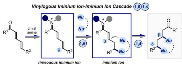
Fig. 9. Vinylogous iminium ion (1,6)/iminium ion (1,4) cascade pathway; the blue and grey circles represent the chiral scaffolds of the aminocatalyst.
