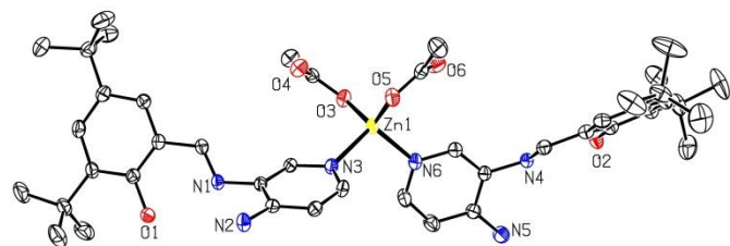
Fig. 1 X-ray molecular structure (ball and stick representation) for complex 3 , co-crystallized solvent molecules and H-atoms are omitted for clarity. Only one molecule of the asymmetric unit is shown here. Selected bond distances (Å) and angles (°) with esd's in parentheses: Zn(1)-O(3) = 1.950(2), Zn(1)-O(5) = 1.963(2), Zn(1)-N(3) = 2.044(3), Zn(1)-N(6) = 2.018(3); N(6)-Zn(1)-N(3) = 106.02(11), O(5)-Zn(1)-O(3) = 123.88(10), N(6)-Zn(1)-O(5) = 114.84(11), N(3)-Zn(1)-O(3) = 107.37(10).
