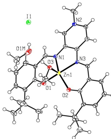
Fig. 3 X-ray molecular structure for 7 . Note that only one molecule is shown from the unit cell. Selected bond distances (Å) and angles (°) with esd's in parentheses: Zn(1)-O(1) = 1.943(2), Zn(1)-O(2) = 1.962(2), Zn(1)-N(1) = 2.057(2), Zn(1)-N(3) = 2.086(2), Zn(1)-O(3) = 2.091(2); N(1)-Zn(1)-N(3) = 79.46(9), O(1)-Zn(1)-O(2) = 95.83(9), N(1)-Zn(1)-O(2) = 154.15(9), N(1)-Zn(1)-O(1) = 90.37(9), N(3)-Zn(1)-O(1) = 163.44(9), N(3)-Zn(1)-O(2) = 88.12(9), N(3)-Zn(1)-O(3) = 96.24(9), O(1)-Zn(1)-O(3) = 98.96(9).
