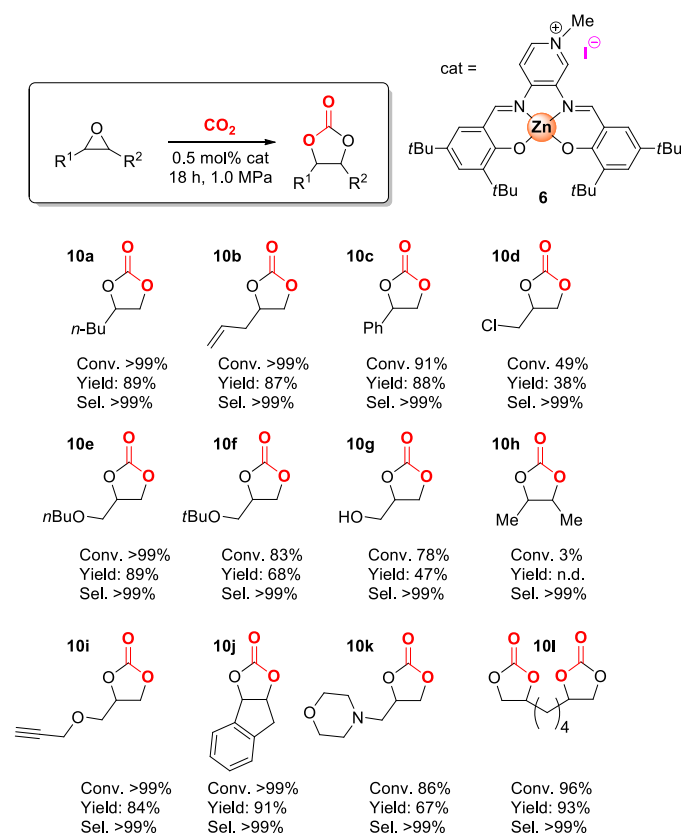
Fig. 4 Substrate scope with Zn(salpyr) complex 6 . General conditions: 10 mmol substrate, 0.5 mol% 6 , p\text{CO}_2 = 1.0 \text{ MPa} , 18 h, 80^\circ\text{C} , neat. N.d. stands for not determined. The reported yields represent isolated yields after chromatographic purification.
