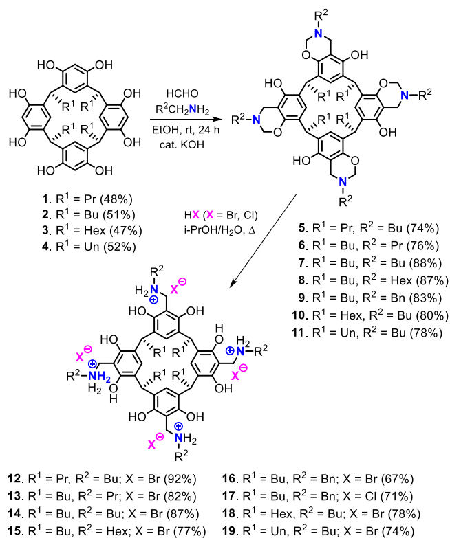
Scheme 1 Synthesis of bifunctional resorcinarene derivatives and their isolated yields.
