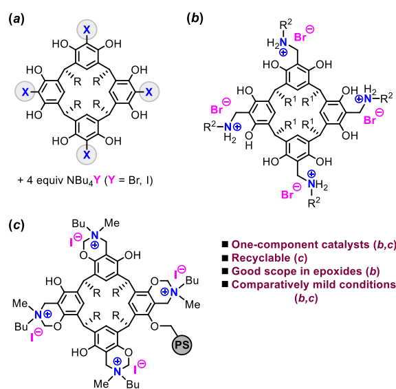
Fig. 1 (a) Previously reported binary resorcinarene (X = H) and pyrogallene (X = OH) catalysts, (b) the bifunctional systems developed in this work, and (c) a heterogeneous version of the bifunctional system (PS = polystyrene).
