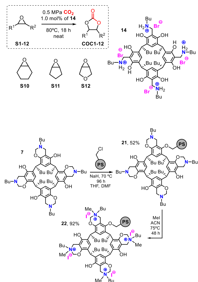
Scheme 2 Synthesis of the bifunctional polystyrene-supported catalyst 22 .
