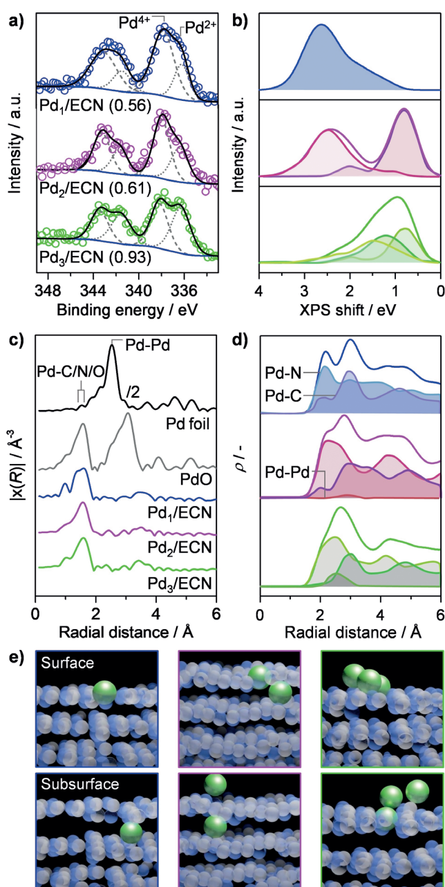
Figure 2. a) Measured and b) simulated Pd 3d core level XPS spectra of the Pd x /ECN catalysts. In (a), black lines show the fits of the raw data (open symbols), gray lines deconvolute the components tentatively assigned to Pd 4+ (dashed) and Pd 2+ (dotted) species, and blue lines show the background. The Pd 2+ :Pd 4+ ratios are indicated in parenthesis. In (b), colored lines represent each Pd atom in the ensemble. c) Normalized k^2 -weighted Fourier Transform of the EXAFS function of the Pd x /ECN catalysts and reference compounds. d) Sum of the radial distribution functions over all the structures generated during the BOMD runs, with the Pd atoms as the reference for Pd x /ECN. e) Snapshots from the BOMD simulations (Supporting Movies 1–3) illustrating distinct possible surface and subsurface configurations of metal ensembles. Green Pd, pale blue N, and grey C.
