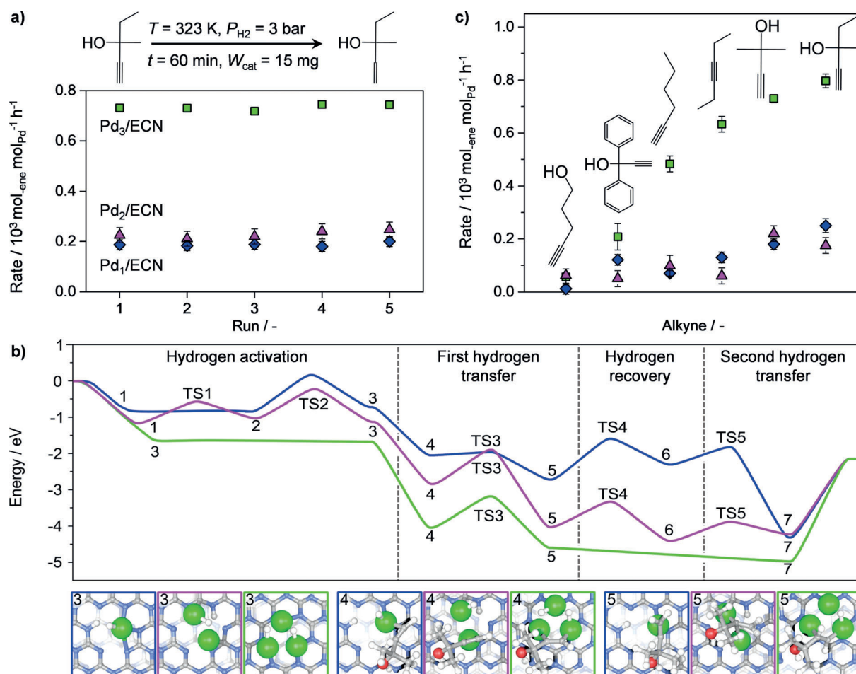
Figure 3. a) Variation in the rates of 2-methyl-3-buten-2-ol formation in the hydrogenation of 2-methyl-3-butyne-2-ol (depicted) over five sequential runs and b) the calculated reaction paths over the surface configurations (with all atoms at the surface) of the Pd ensembles in Pd x /ECN. Green Pd, gray C, blue N, red O, and white H atoms. TS=transition state. c) Rates of alkene formation in the hydrogenation of distinct functionalized alkynes (illustrated). The color code for data points in (a) applies to (b) and (c).
