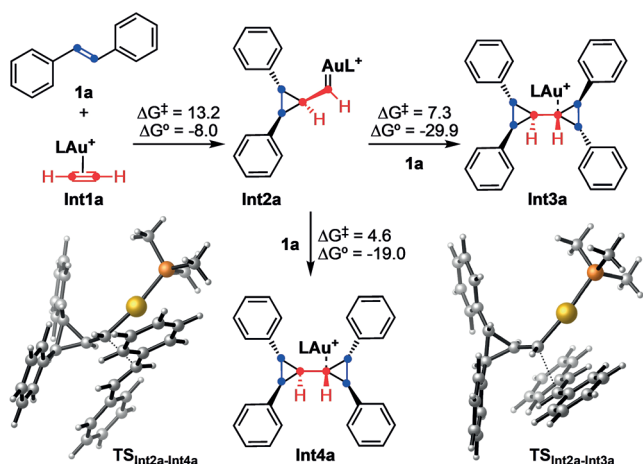
Scheme 4. Calculated formation of different diastereomers of bicyclopropyl products. L = \text{PMe}_3 . DFT calculations performed with M06-D3/6-31G(d) (C, H, P) and SDD (Au) in \text{CH}_2\text{Cl}_2 (SMD). Free energies in \text{Kcal mol}^{-1} .
