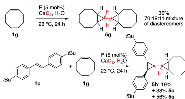
Scheme 3. Bicyclopopylation of cyclooctene.
