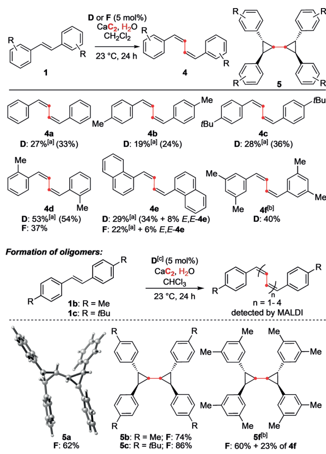
Scheme 2. Synthesis of dienes 4 and bicyclopopyl compounds 5 from acetylene and stilbenes 1a–f and oligomerization experiments. Yields of isolated products (yields determined by 1 H NMR using diacetyl benzene as internal standard in parenthesis); 5a is shown as a CYLview depiction of the X-ray crystal structure. [a] Isolated as a mixture with starting material. [b] Reaction carried out in chloroform, at 40 °C. [c] Reaction with equimolar amounts of t BuXPhosAuCl and NaBAr F 4 .
