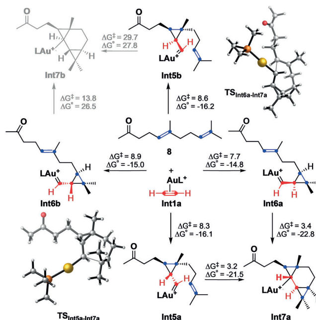
Scheme 7. Different mechanistic pathways to form Int7a,b by double cyclopropanation reactions. L = \text{PMe}_3 . DFT calculations performed with M06-D3/6-31G(d) (C, H, P, O) and SDD (Au) in \text{CH}_2\text{Cl}_2 (SMD). Free energies in \text{kcal mol}^{-1} .
